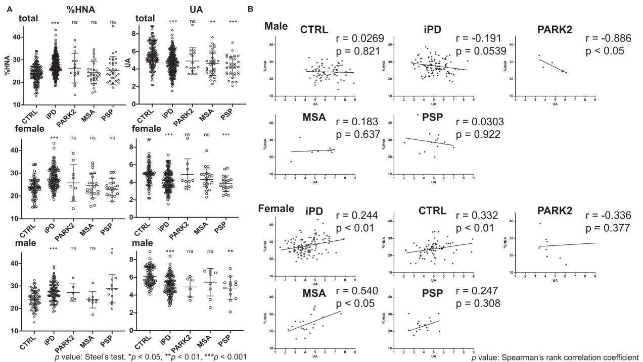
Figure 4. Association between %HNA and UA, which is an antioxidant compound. (A) Analysis of UA in all groups and in each sex. (B) Analysis of the correlation between UA and %HNA in each sex. %HNA: the ratio of human nonmercaptalbumin to human serum albumin, UA: uric acid, iPD: idiopathic Parkinson's disease, CTRL: control subject, MSA: multiple system atrophy, PSP: progressive supranuclear palsy, ns: not significant.
