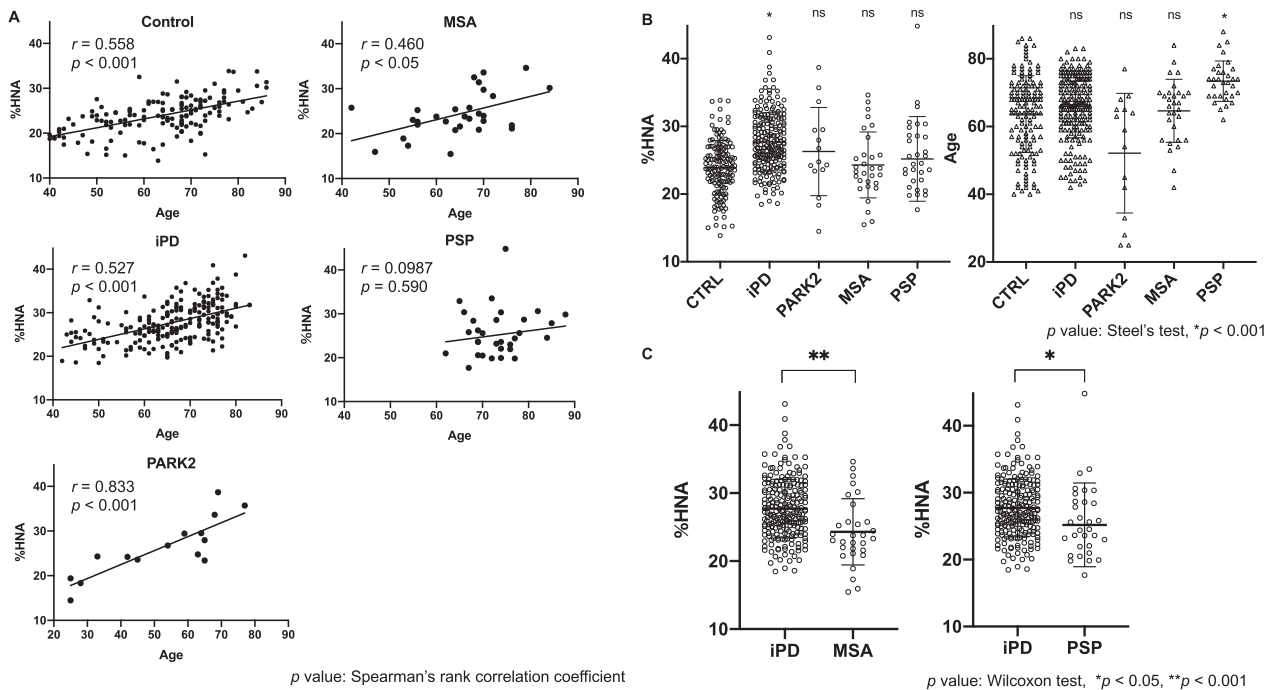
Figure 1. %HNA was positively correlated with age and was higher in iPD patients than in controls. (A) %HNA was positively correlated with age in each group, except for the PSP group. (B) %HNA was higher in the iPD group than the controls. Mean values are displayed. (C) %HNA was higher in the iPD group than in the MSA and PSP groups. %HNA: the ratio of human nonmercaptalbumin to human serum albumin, iPD: idiopathic Parkinson's disease, CTRL: control subject, MSA: multiple system atrophy, PSP: progressive supranuclear palsy, ns: not significant.
