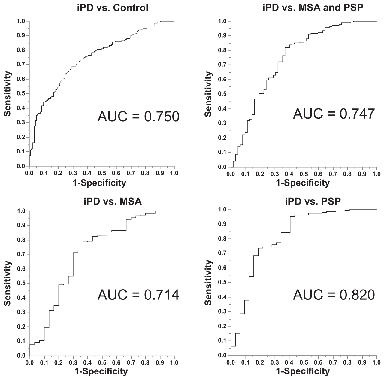
Figure 3. %HNA may be a reliable biomarker for distinguishing iPD patients from controls and MSA and PSP patients. The ROC curve and corresponding AUC were analyzed using the Youden index. The optimal cutoff point was measured by the maximum sensitivity and specificity. % HNA: the ratio of human nonmercaptalbumin to human serum albumin, iPD: idiopathic Parkinson's disease, CTRL: control subject, MSA: multiple system atrophy, PSP: progressive supranuclear palsy, ROC: receiver operating characteristic, AUC: area under the curve.
