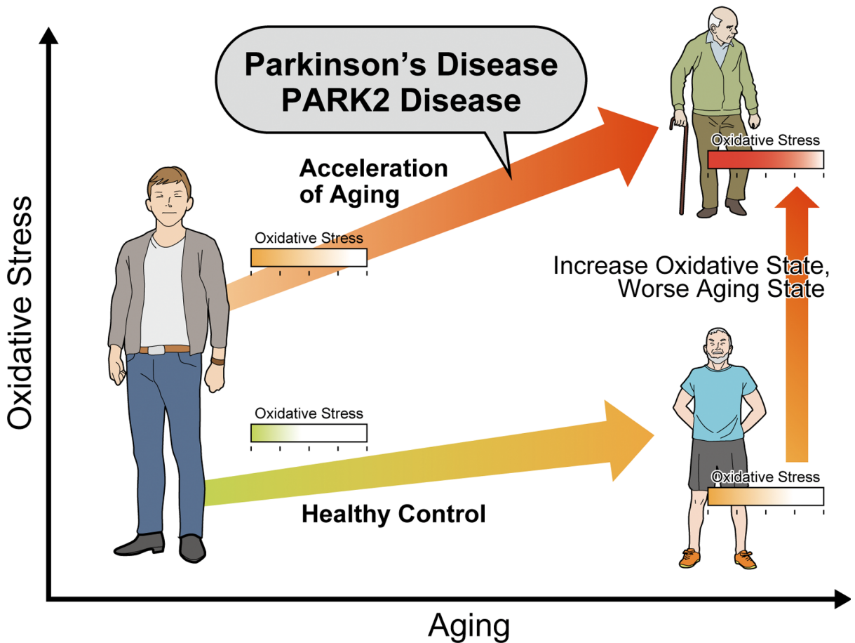
Figure 5. Elevated levels of the oxidized form of albumin accelerate aging and affect the pathomechanisms of Parkinson's and PARK2 disease. (A) Human serum albumin is converted from the reduced form to the oxidized form by oxidative stress in the whole body. (B) Elevation of oxidative stress may accelerate aging and affect the pathomechanisms of Parkinson's and PARK2 disease.
