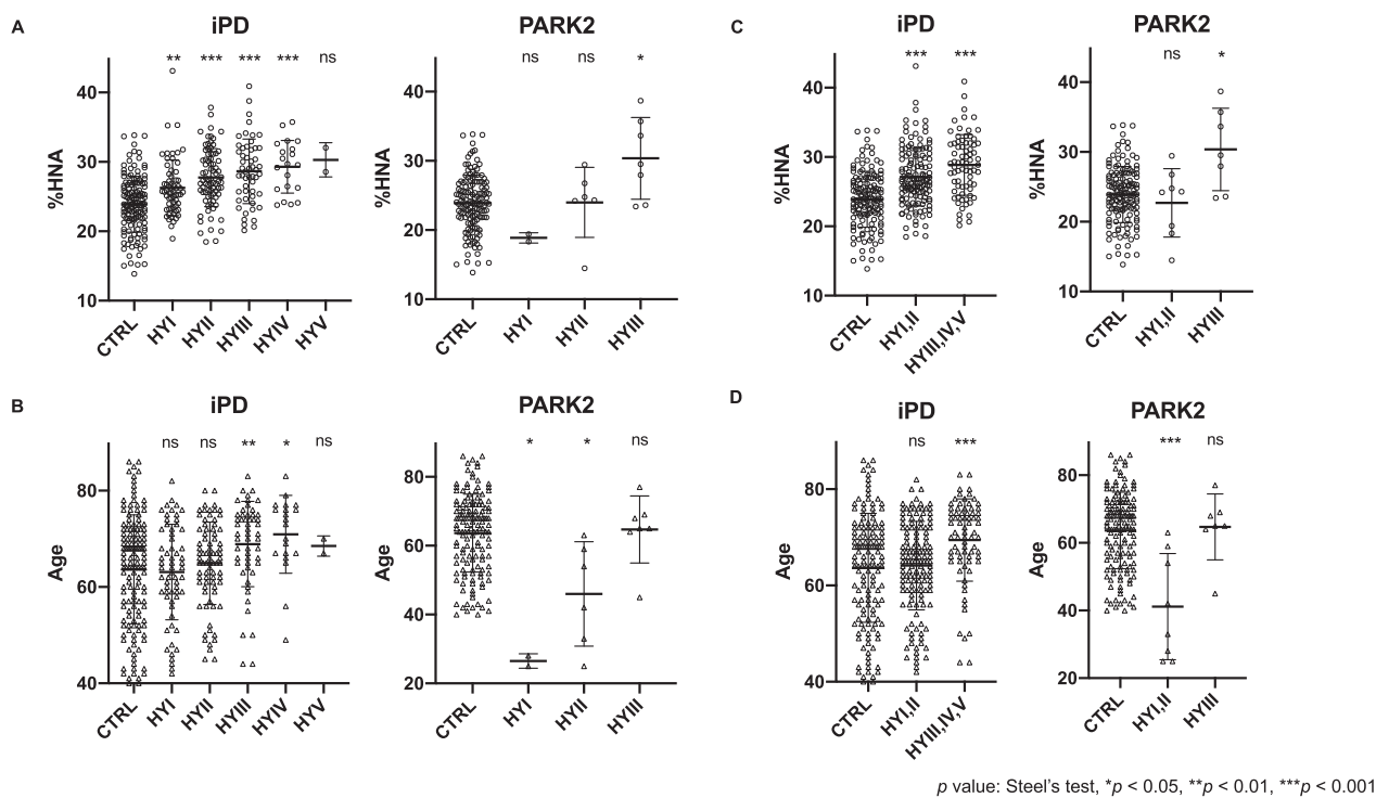
Figure 2. Correlation between %HNA and disease severity. (A–D) To compare controls and patients with iPD and PARK2 for disease severity, we classified patients by H&Y stage into two groups: a mild group (H&Y I, II) and a severe group (H&Y III, IV, V). %HNA: the ratio of human nonmercaptalbumin to human serum albumin, iPD: idiopathic Parkinson's disease, CTRL: control subject, H&Y: Hoehn & Yahr, ns: not significant.
